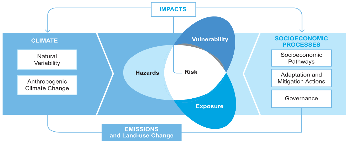
Figure 1.37: Illustration of the core concepts of IPCC WGII AR5
