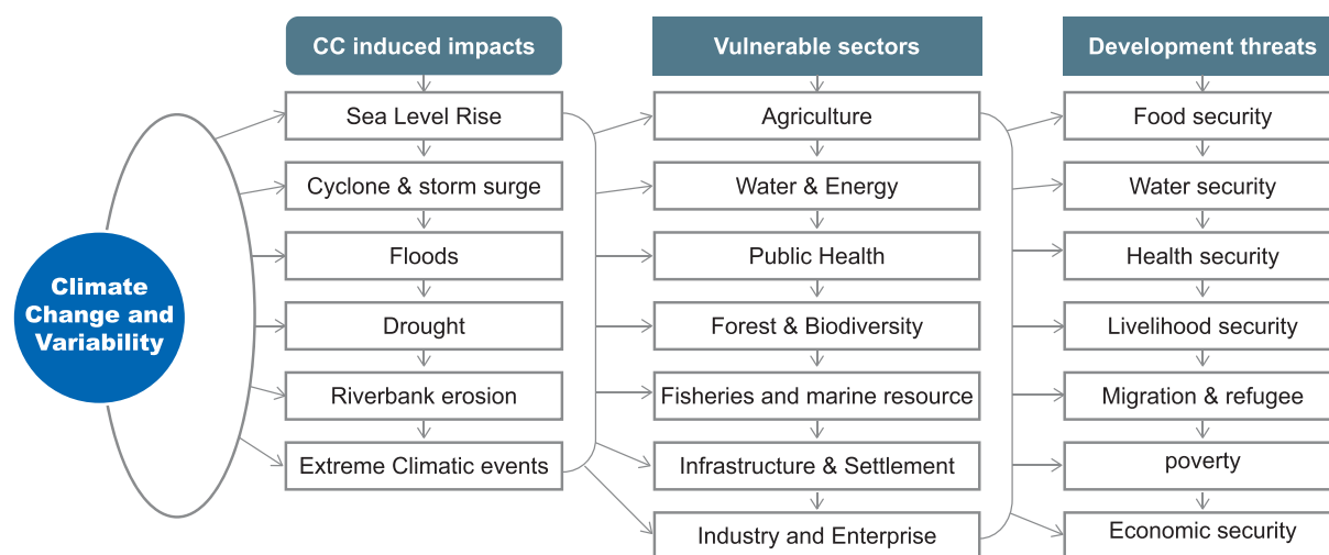
Figure 1.36: Impact Vulnerability and Development Linkage
