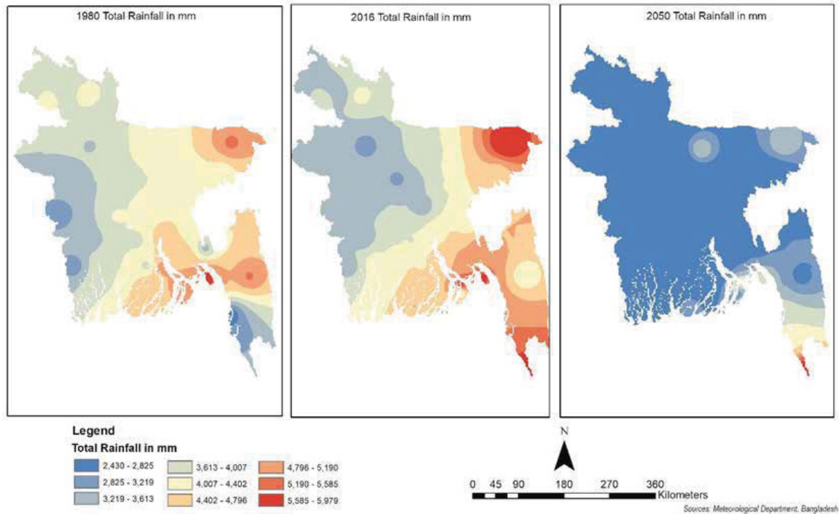
Figure 3.6: Bangladesh total rainfall and prediction
