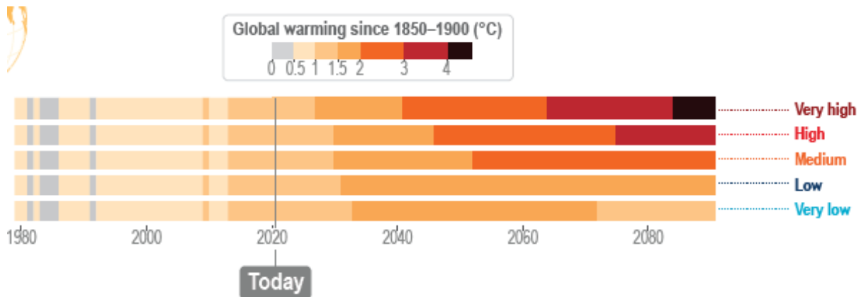
Figure 1.20: Effect on surface temperature
