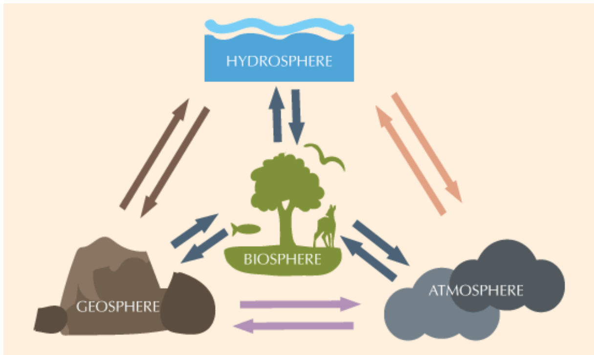
Figure 1.3: Climate Systems
