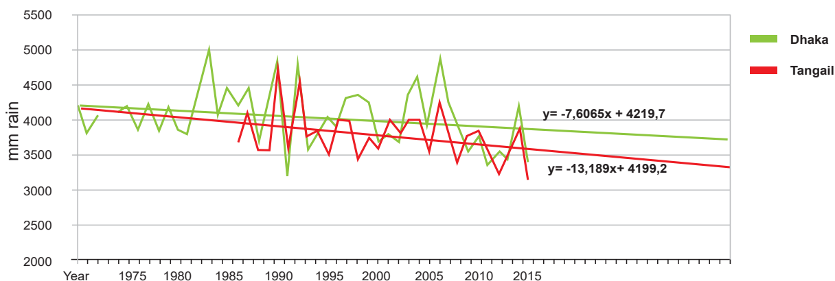
Figure 3.4: Historical precipitation data & trendline
