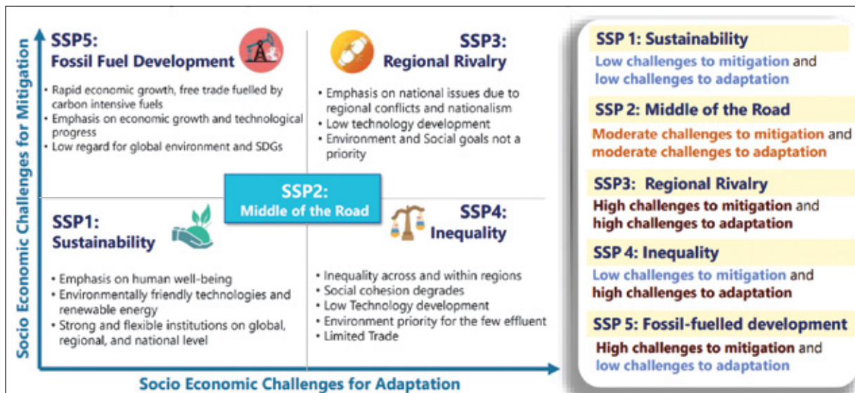
Figure 1.17: Characteristics of SSPs
