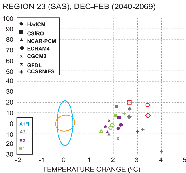
Figure 3.2: Scatter plot projections
