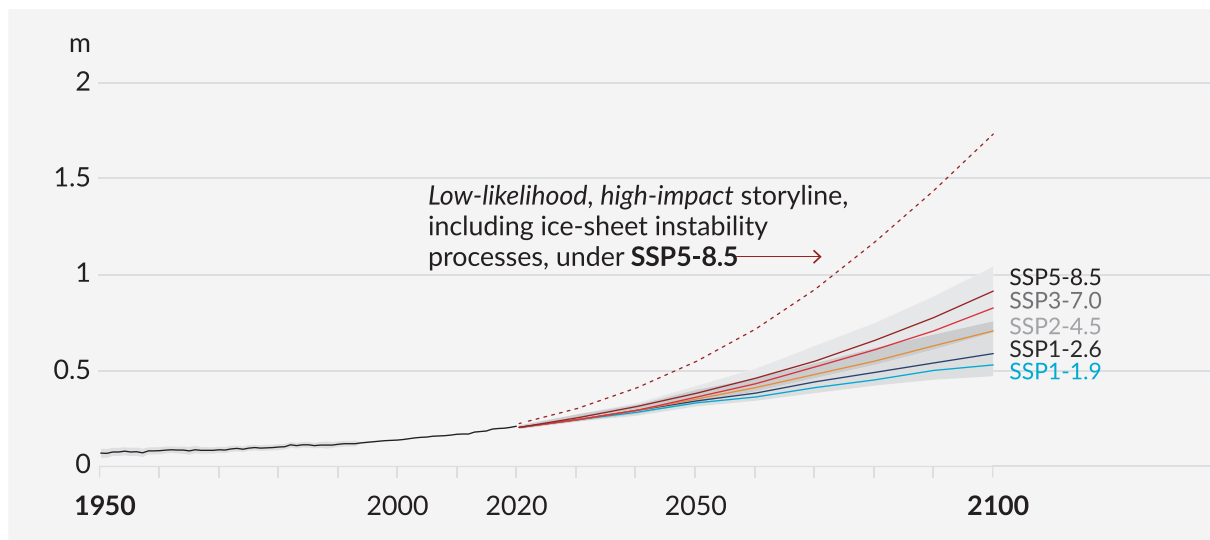
Figure 1.12: Global mean sea level change relative to 1900 (IPCC AR6, 2021)
