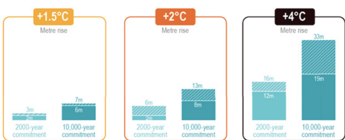
Figure 1.22: Long-term consequences: Sea Level Rise
