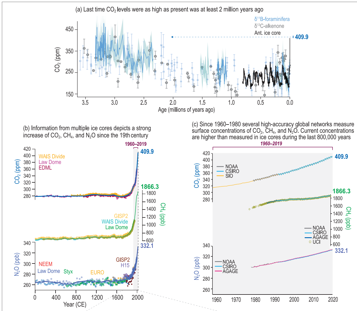
Figure 1.9: Changes in well-mixed greenhouse gas (WMGHG) concentrations (IPCC AR6, 2021)
