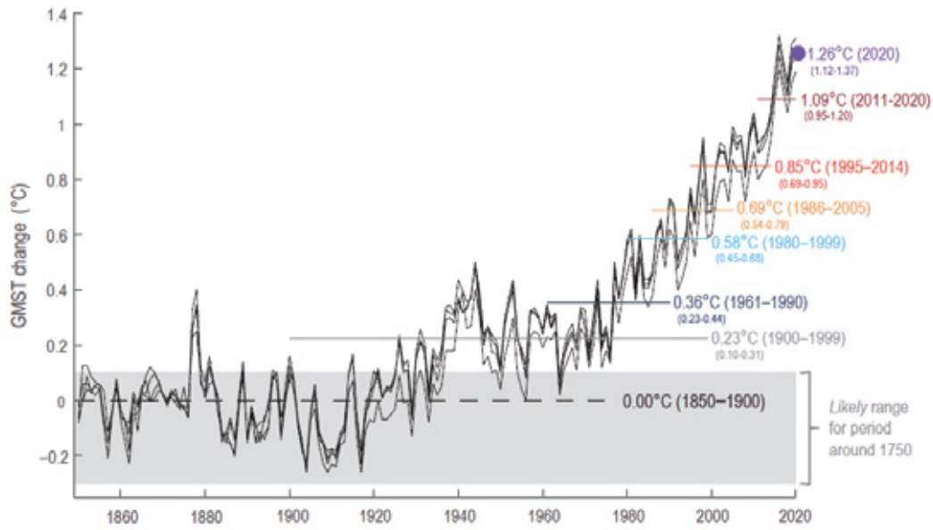
Figure 1.10: Global Warming over the Instrumental Period
