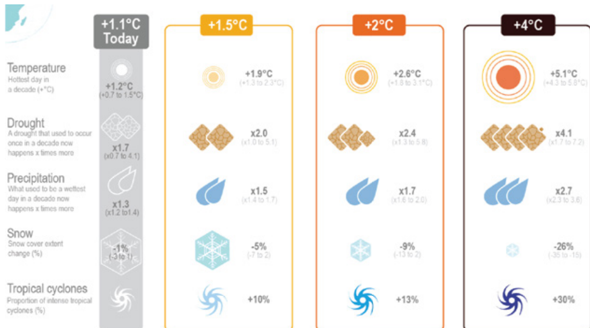
Figure 1.21: Response of the climate system relative to 1850–1900
