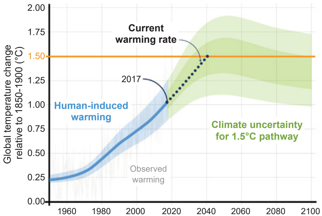
Figure 1.11: Human-induced warming reached approximately 1°C above pre-industrial levels in 2017 (Source: Global warming of 1.5°- IPCC special report)
