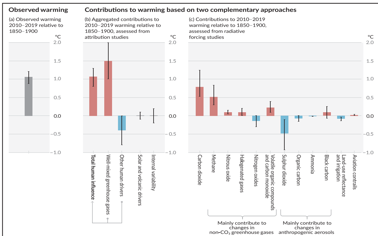
Figure 1.6: Assessed contributions to observed warming in 2010–2019 relative to 1850–1900
