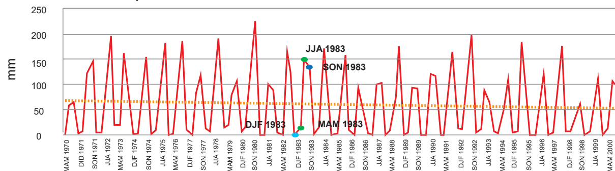
Figure 3.1: Scatter Plot Projections
