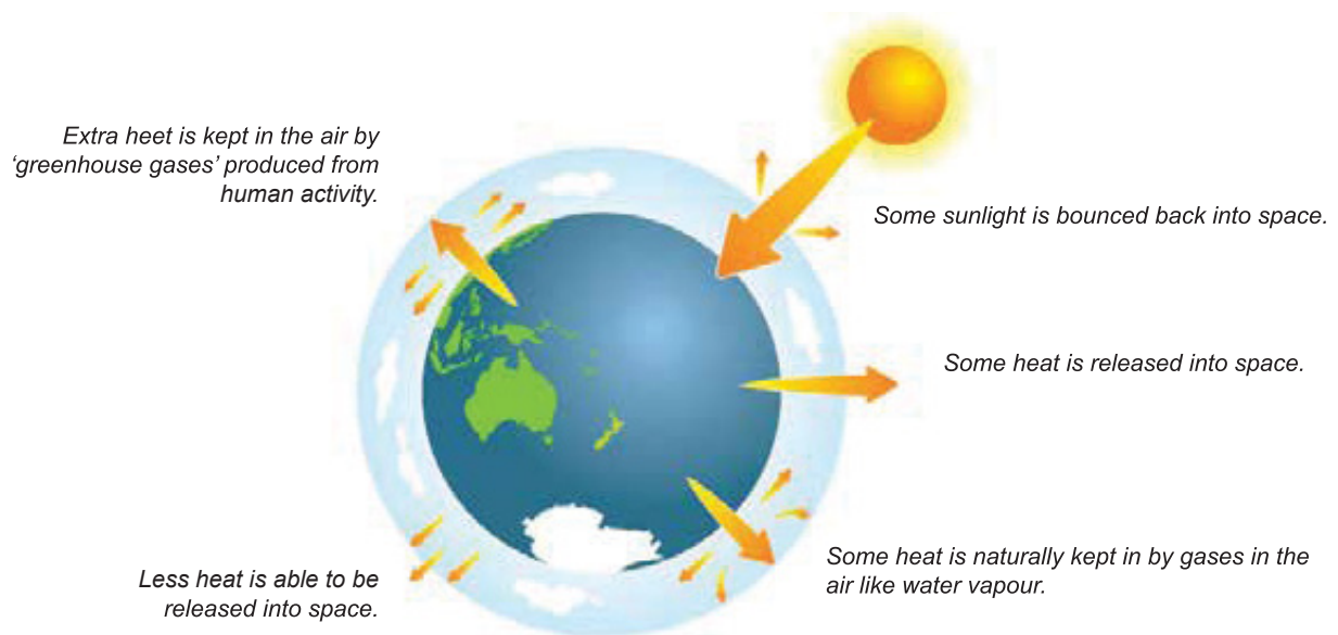
Figure 1.5: Greenhouse effect in Earth's Atmosphere
