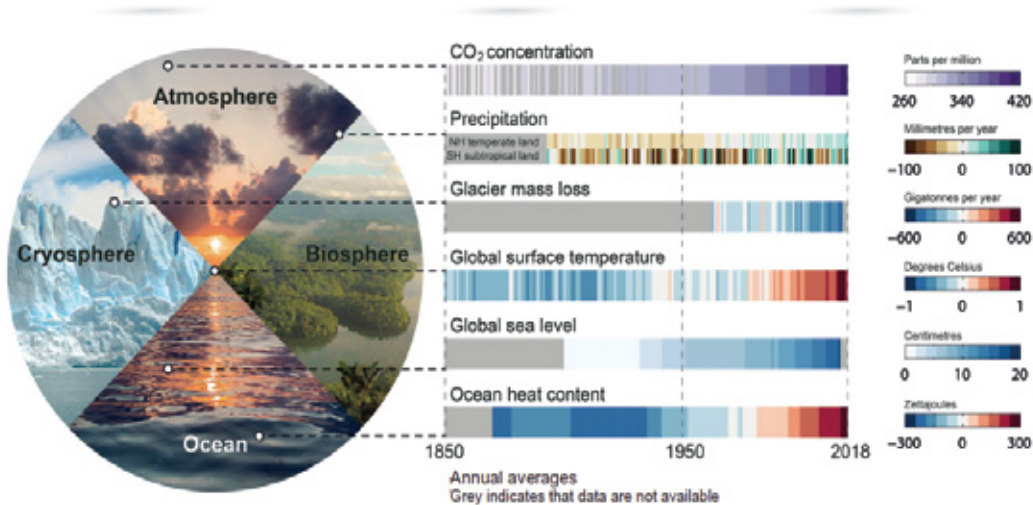
Figure 1.7: Changes in Occurring throughout the Climate System, IPCC AR6-2021
