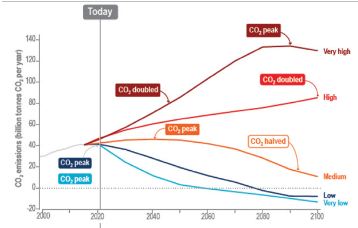
Figure 1.19: Emission Pathways
