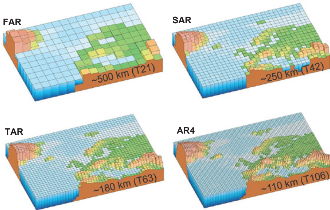
Figure 1.18: Improvement of Climate Model Resolution from IPCC FAR to AR4
