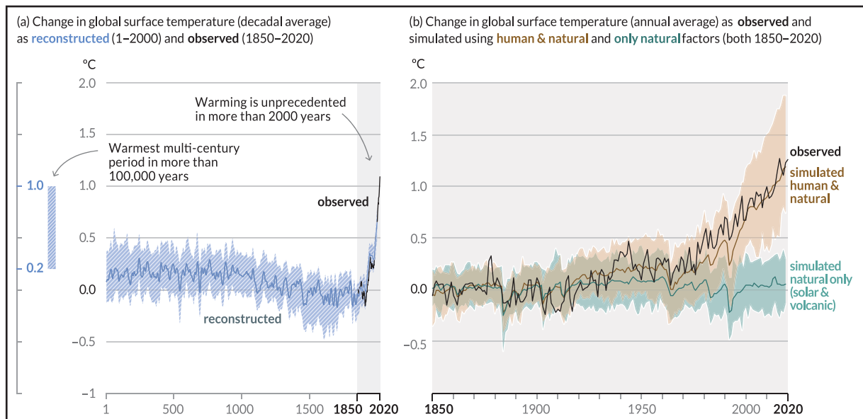
Figure 1.4: Changes in global surface temperature relative to 1850–1900 (unprecedented temperature increase by human activities in the last 2000 years).
