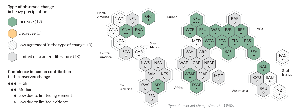
Figure 1.13: Synthesis of assessment of observed change in heavy precipitation and confidence in human contribution to the observed changes in the world's regions (IPCC AR6, 2021).
