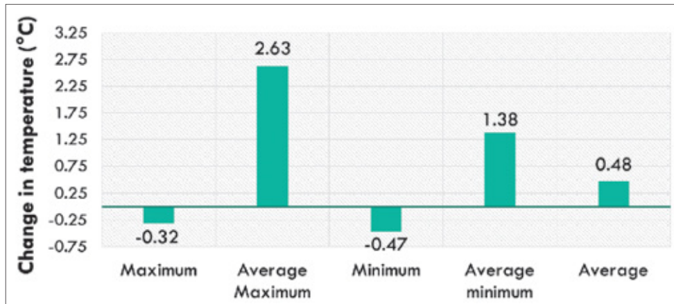
Figure 1.14: Decadal Changes in Average Temperature
