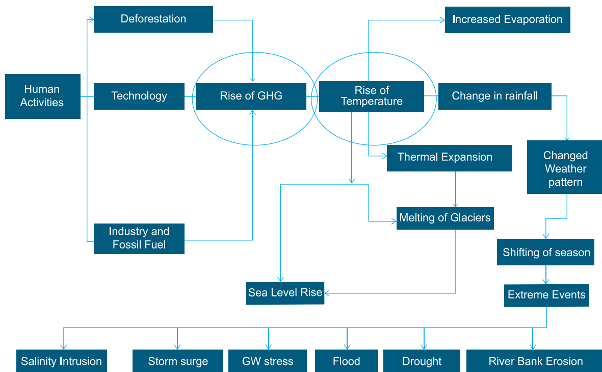
Figure 1.8: Climate Change Process
