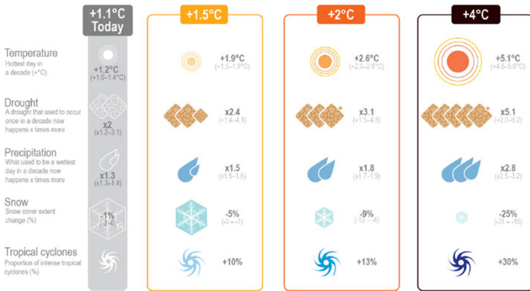
Figure 2.17: Change in the frequency of extreme temperature, drought, heavy precipitation, snow cover, and proportion of tropical cyclones (source: IPCC, 2021)
