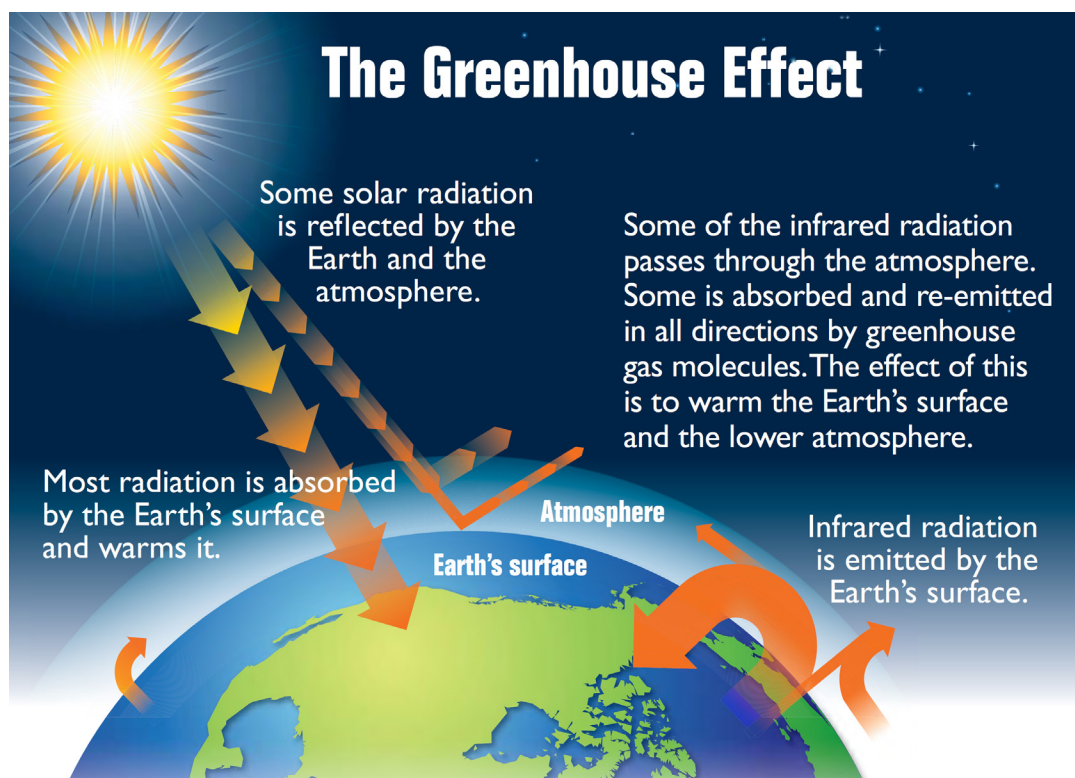
Figure 1.2: Schematic diagram of the greenhouse effect (source: Energy Education, 2021)
