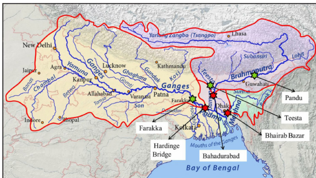
Figure 1.10: The boundary of the Ganges–Brahmaputra–Meghna (GBM) basin (thick red line), (source: Masood et al. 2015)
