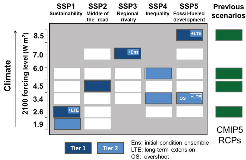
Figure 2.12: Shared socio-economic pathways (SSPs) and representative concentration pathways (RCPs) (source: O'Neill, 2016)
