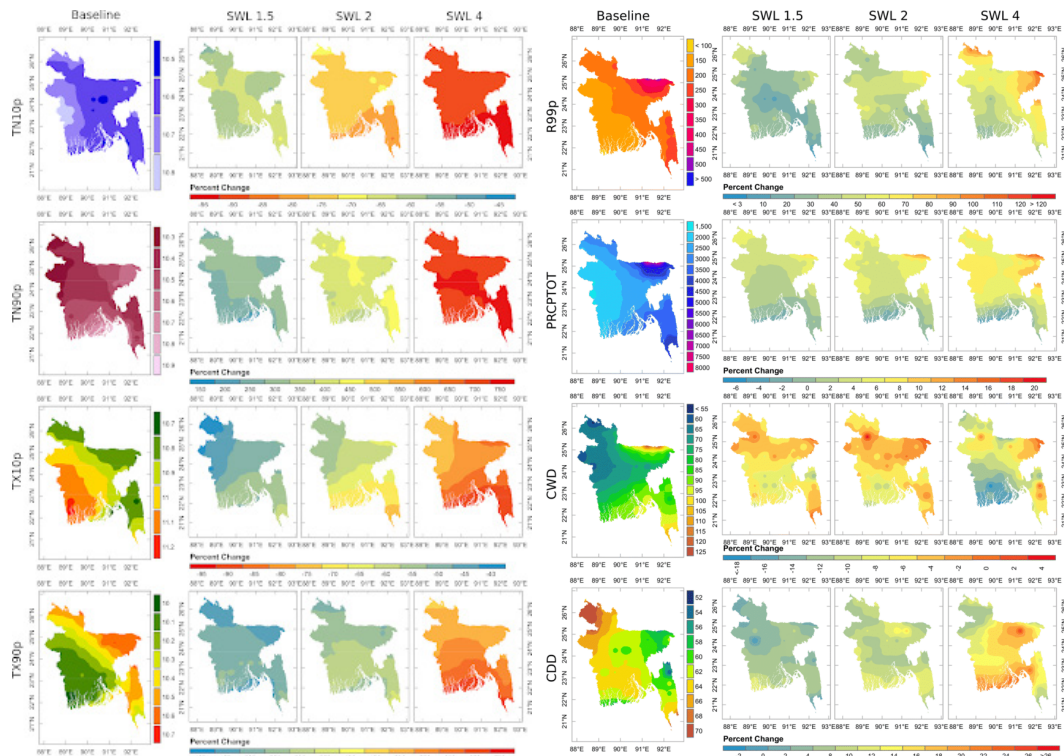
Figure 2.21a: Spatial distribution and percentage change in cold nights (TN10p), warm nights (TN90p), cold days (TX10p), and warm days (TX90p) (source: Khan et al., 2020)
