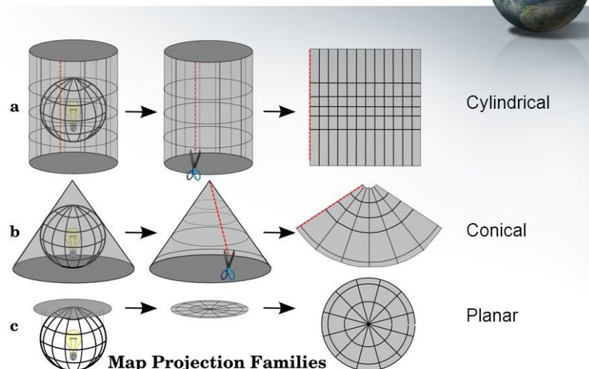
Figure 12.16: Projected coordinate system (Source: ASPEXIT, 2020)
