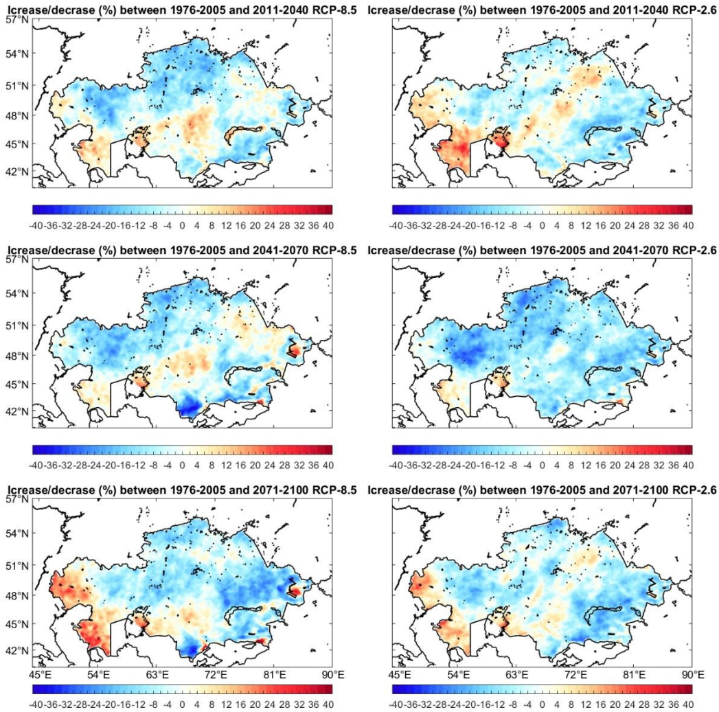
Figure A6. Extreme wind speed evolution in the 21 st century. The left panels show the evolution under RCP 8.5 scenario and the right panels under RCP 2.6 scenario. The top panels show the average increase/decrease (in %) of the number of events per year with respect to the historical period by the beginning of the century, the center panels by midcentury and the bottom panels by the end on the century.
