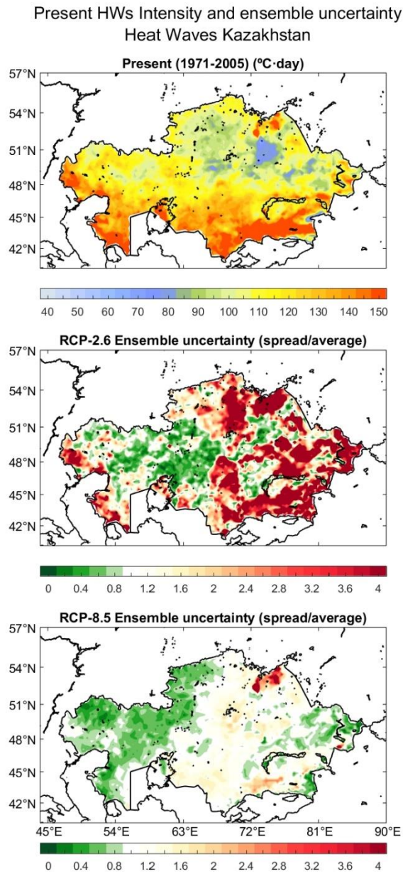
Figure A9. The top panel shows the average intensity of the heatwaves in the historical period ( ^{\circ}\text{C}\cdot\text{day} ). The central and bottom panels show the ensemble uncertainty for the RCP 2.6 and RCP 8.5 scenarios, respectively.
