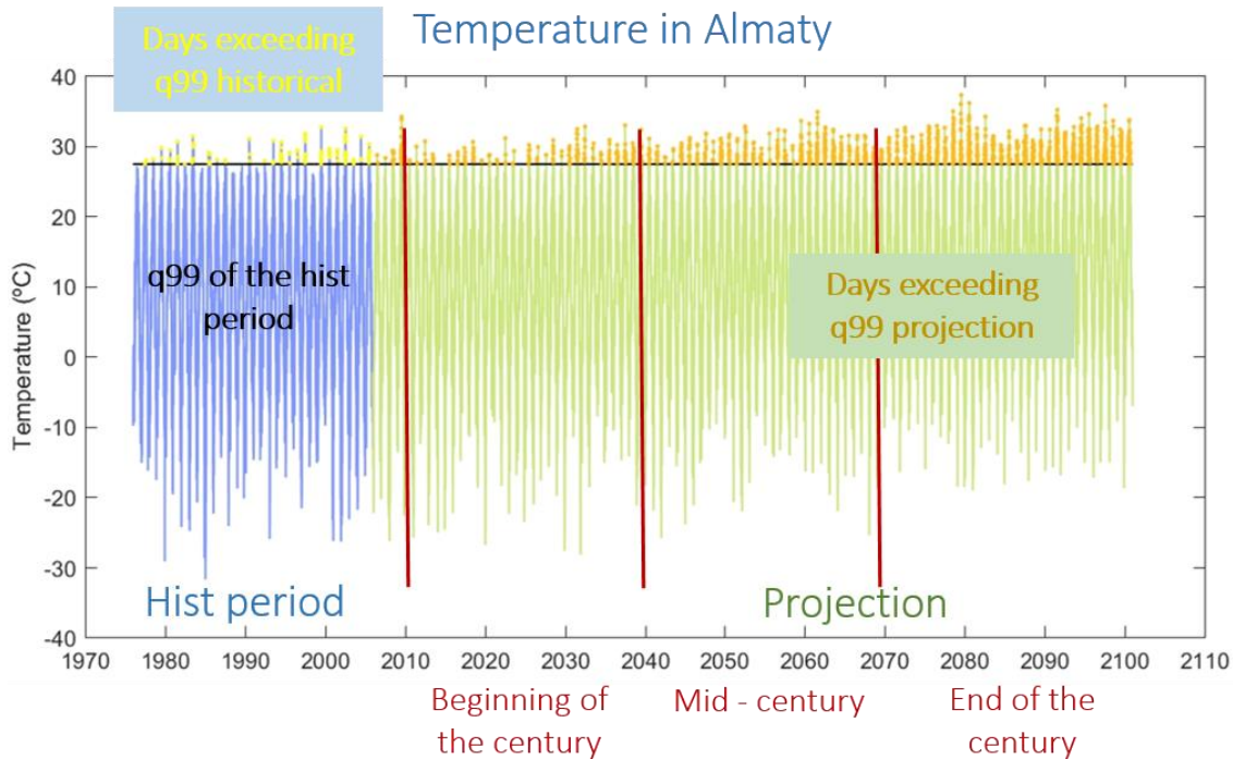
Figure 7. Time series of the temperature in the grid point closer to Almaty. The blue line corresponds to the historical period and the green line to the RCP 8.5 projection. The black horizontal line is the q99 threshold of the historical period. Yellow points indicate the values of extreme temperature over the historical period and orange points over the projection. The three vertical red lines mark the limits of the three time horizons considered: beginning of the century (2011-2040), midcentury (2041-2070) and end of the century (2071-2100).
