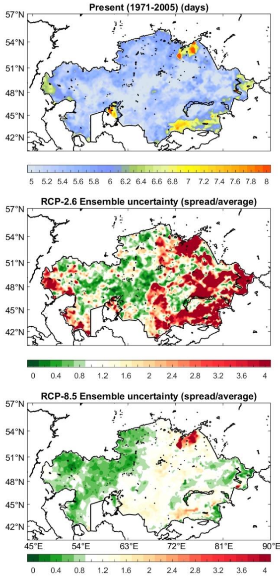
Present HW duration and ensemble uncertainty Heat Waves Kazakhstan
