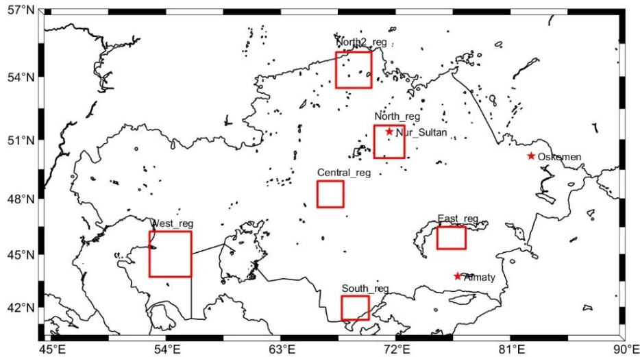
Figure 11. Locations of the point/regions where the yearly time series of the indicators are computed.
