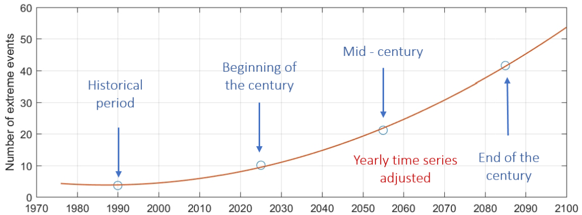
Figure 10. Example of how the yearly time series of the extreme temperature in Almaty is computed for the RCP 8.5 projection. The blue circles represent the average of the number of events per year for the historical period and the three time horizons defined for the 21 st century. The red line is the time series resulting of adjusting the four 30-year averages to a second degree polynomial function.
