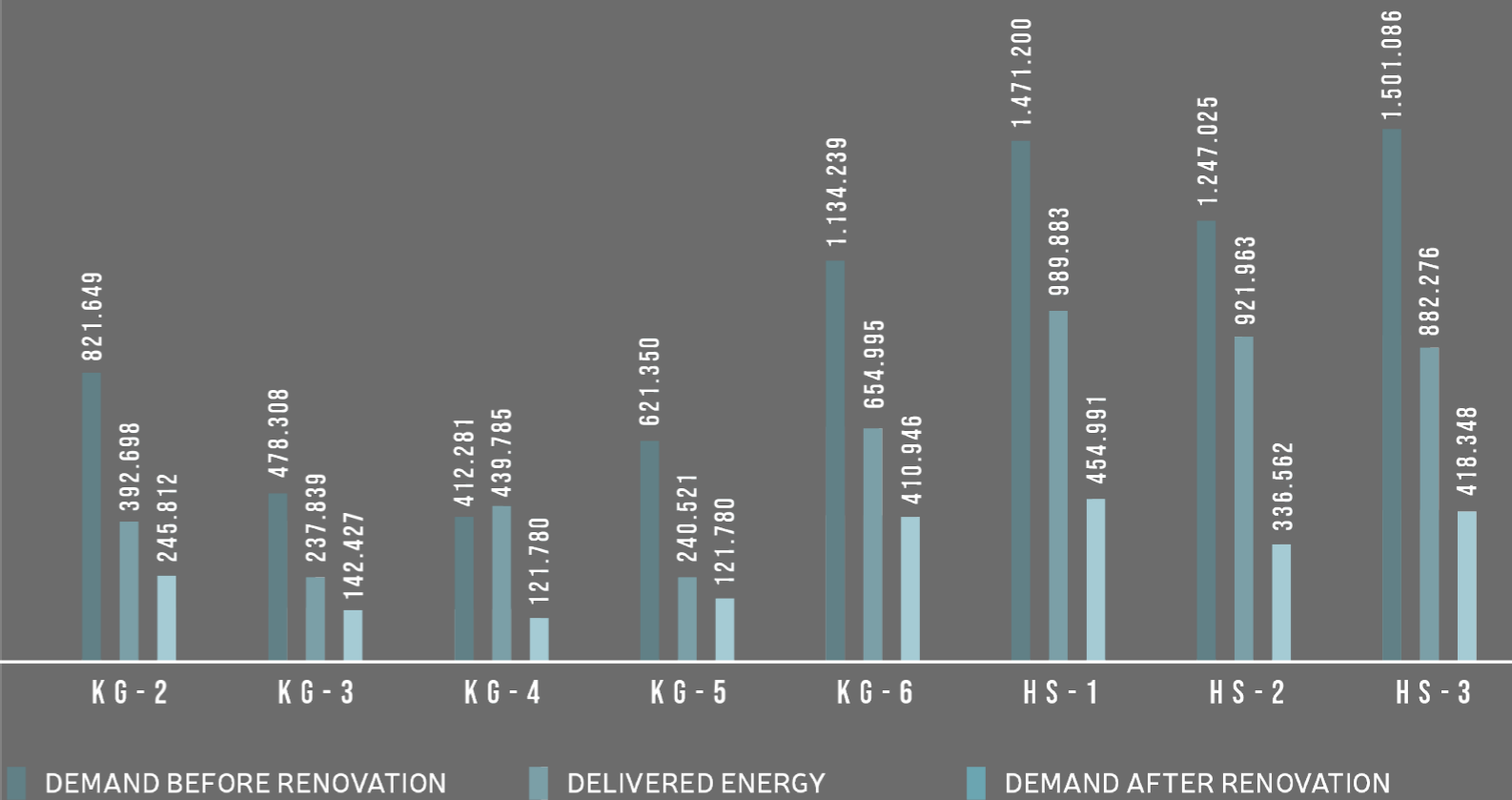
HEATING DEMAND IN kWh/a PER BUILDING TYPE
